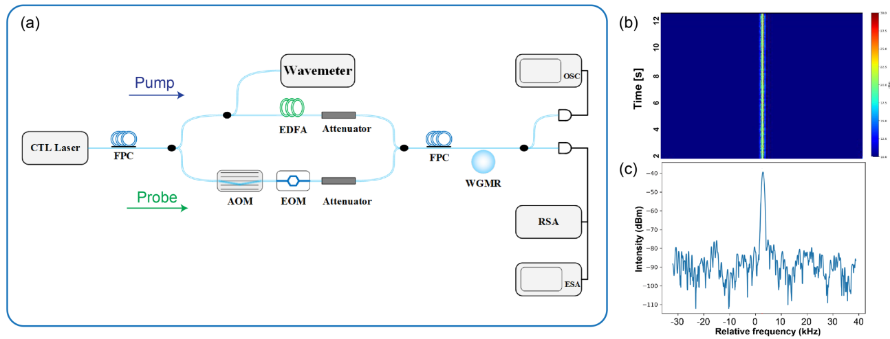
Fig. 3. Experimental setup of optical memory effect of an SBS laser. (a) Schematic illustration of the experimental optical memory effect based on Brillouin laser in a microsphere cavity. The upper optical path is the pump laser; the wavemeter is used to monitor the current wavelength of the pump. The lower optical path is the probe laser modulated to scan across the SBS laser through an electrical-optical modulator (EOM). The acoustic-optical modulator is used to help distinguish between Stokes and anti-Stokes. Time evolution spectrum of SBS laser during probe scanning is recorded by RSA, and the beat frequency spectrum is recorded by an electrical spectrum analyzer (ESA) (b) Two-dimensional spectra of a static SBS laser in frequency (horizontal axis) with time evolution (vertical axis); note that the probe is absent in this case. (c) Beating frequency spectrum of an SBS laser in an electrical spectrum analyzer.
